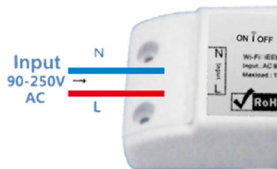
Appliance wiring instruction
